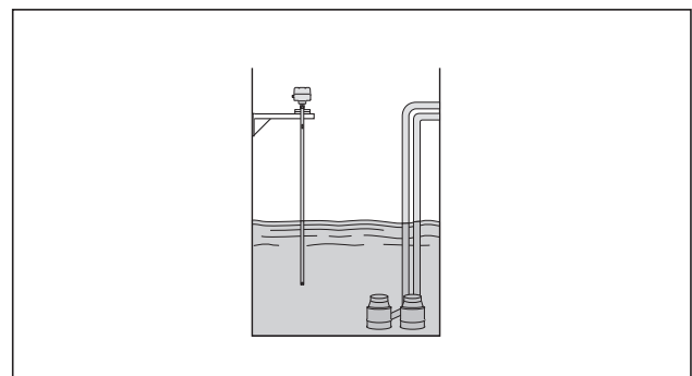
Pump Control
