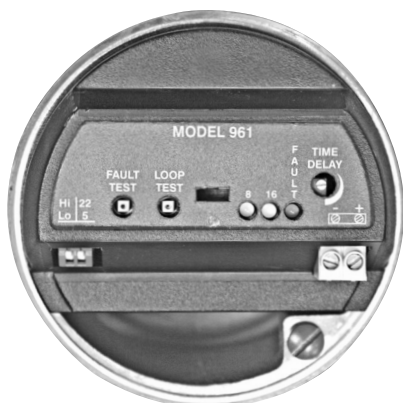
Loop powered 961
